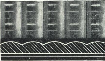
CUTTING NO. 2. Transmits 73.4% of the light falling upon it. 1.36 sq. ft. of this block are equivalent to 1 sq. ft. of ordinary window.
